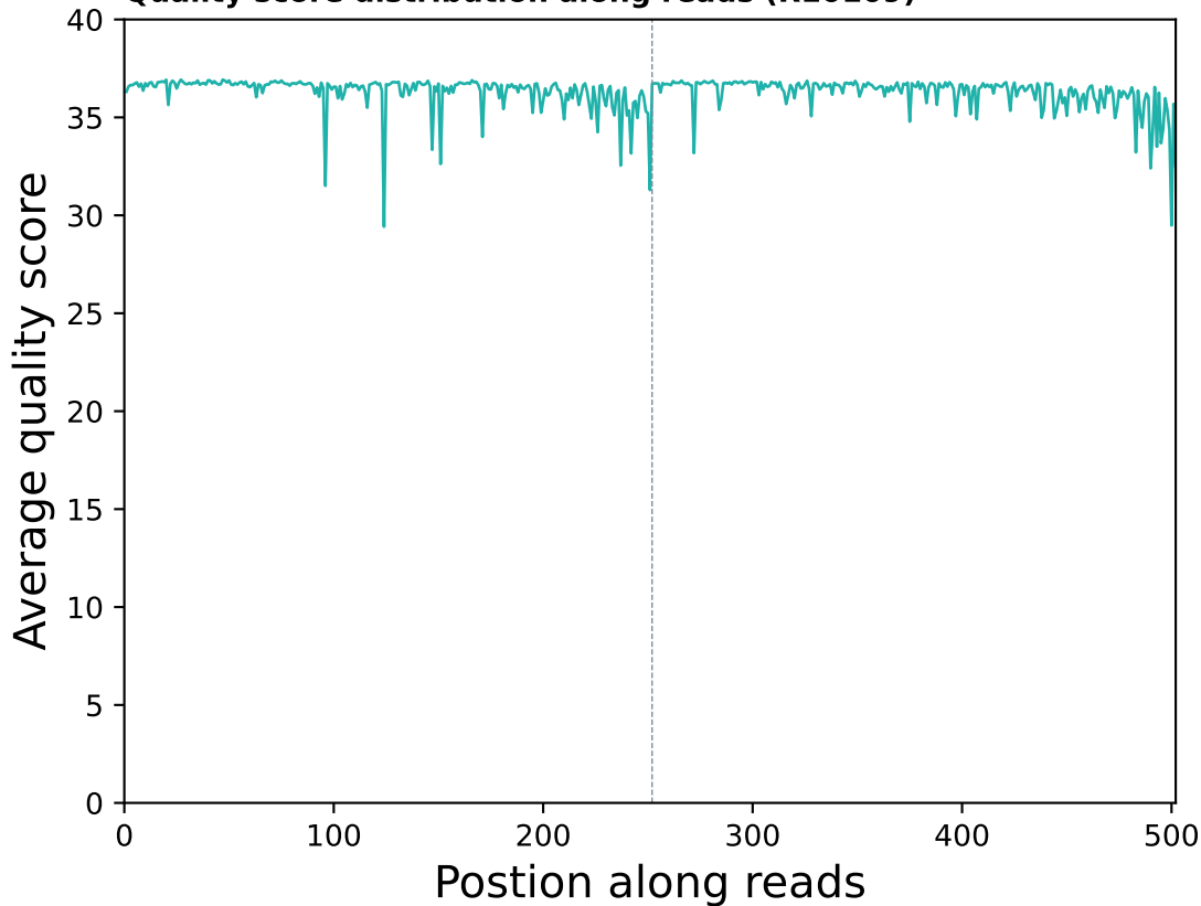
Quality score distribution along reads (R10109)
